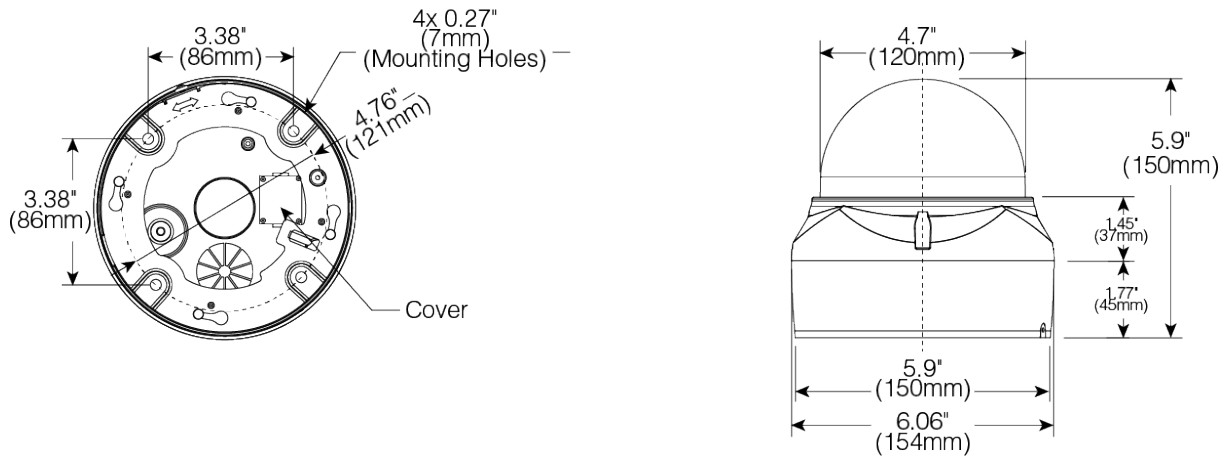
Figure – Dimension
